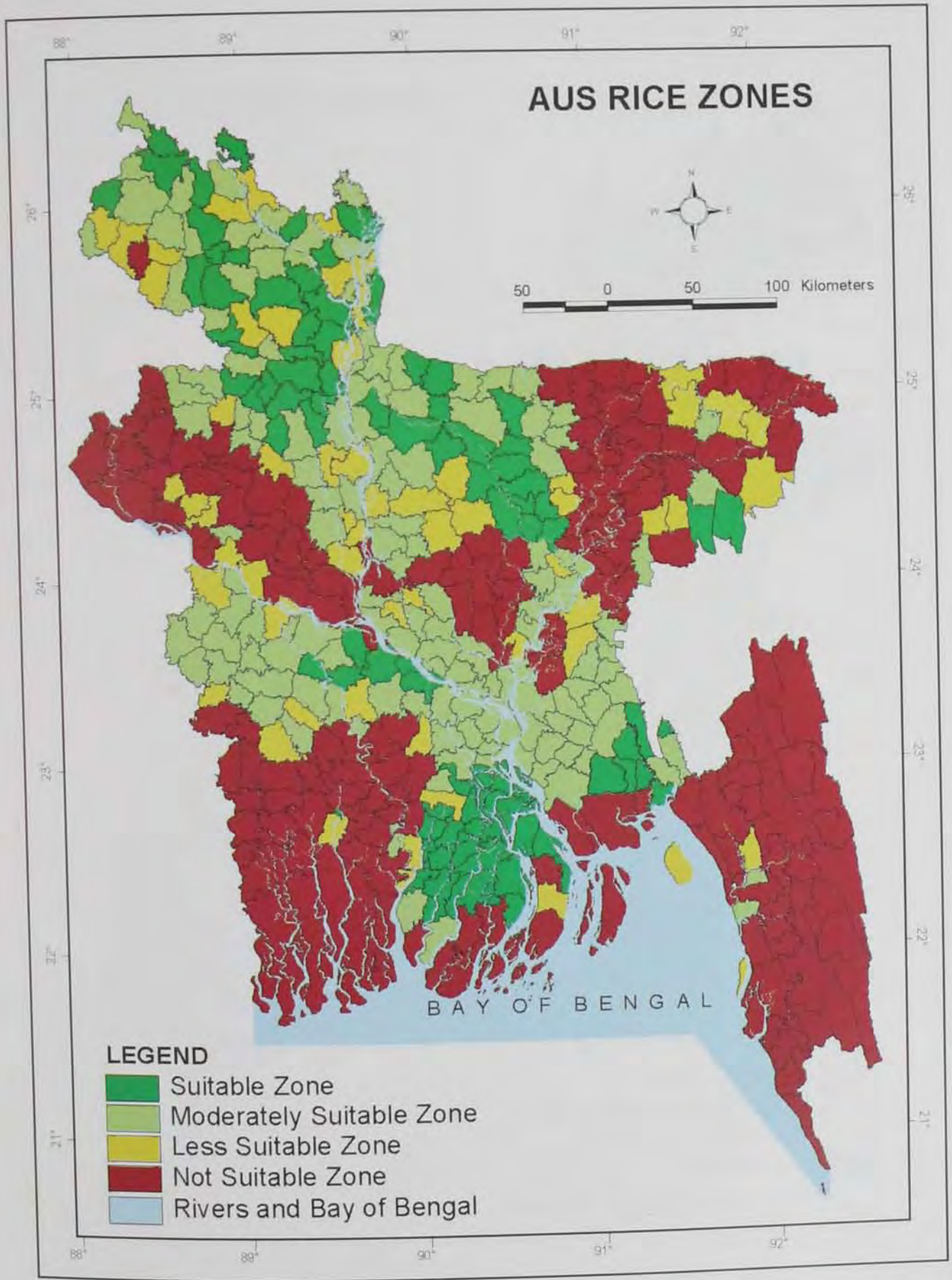
Figure 39. Zones for T. Aus Rice Production
